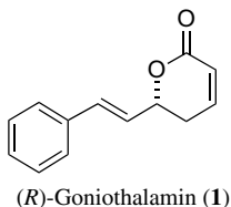
Figure 1. Structure of ( R )-goniothalamine ( 1 ).
