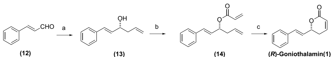
Scheme 3. Conditions: (a) (R,R)-11 [(R)-BINOL (10 mol %), Ti(O i -Pr) 4 (15 mol %), TiCl 4 (5 mol %), Ag 2 O (10 mol %)], allyltributyltin (1.1 equiv), CH 2 Cl 2 , –20 °C, 24 h (94%; 94% ee); (b) acryloyl chloride (1.8 equiv), Et 3 N (3.6 equiv), CH 2 Cl 2 , 0 °C (80%); (c) Grubbs' catalyst [(PCy 3 ) 2 Cl 2 Ru=CHPh] (10 mol %), CH 2 Cl 2 (98%).
