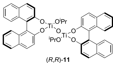
Figure 2. The \mu -oxo bis(binaphthoxy)(isopropoxy)titanium complex (R,R)-11 developed for Maruoka and co-workers. 50
