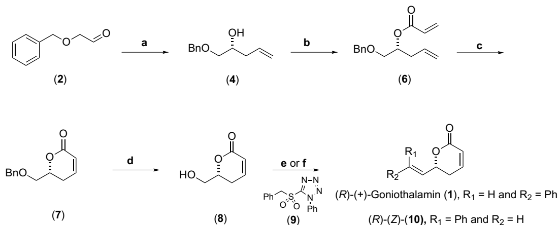
Scheme 2. Conditions: (a) ( R )-BINOL (10 mol %), \text{Ti}(\text{O}i\text{-Pr})_4 (10 mol %), molecular sieves (4 Å), allyltributyltin, -20^\circ\text{C} , 60 h (78%; 94% ee); (b) acryloyl chloride, \text{Et}_3\text{N} , \text{CH}_2\text{Cl}_2 , 0^\circ\text{C} (86%); (c) Grubbs' catalyst [ (\text{PCy}_3)_2\text{Cl}_2\text{Ru}=\text{CHPh} ], \text{CH}_2\text{Cl}_2 (91%); (d) \text{FeCl}_3 , \text{CH}_2\text{Cl}_2 (88%); (e) (\text{COCl})_2 , \text{CH}_2\text{Cl}_2 , DMSO, \text{Et}_3\text{N} , -65^\circ\text{C} , 30 min; then \text{Ph}_3\text{P}=\text{CHPh} , THF (53%, two steps); (f) (\text{COCl})_2 , \text{CH}_2\text{Cl}_2 , DMSO, \text{Et}_3\text{N} , -65^\circ\text{C} , 30 min; then solution of the 9 , KHMDS, THF, -78^\circ\text{C} (<20%).
